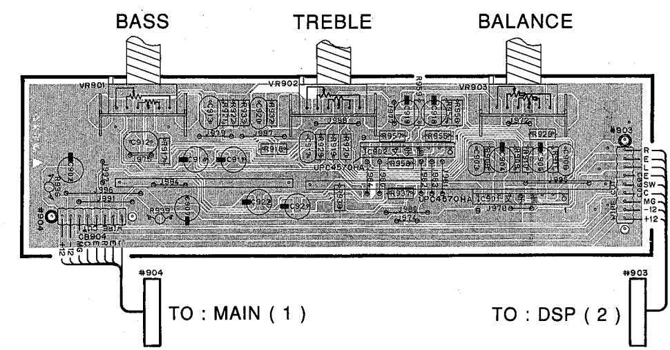
P.C.B. OPERATION ( 2 )
